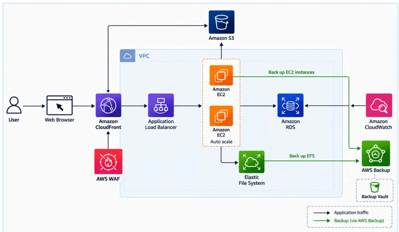
AWS Solution Architecture
